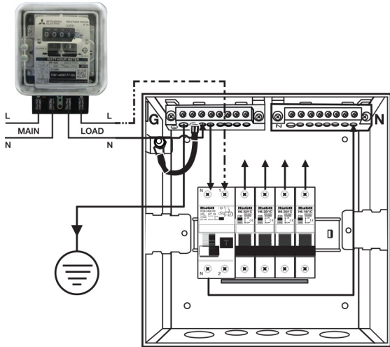
Main RCBO (RO8)
