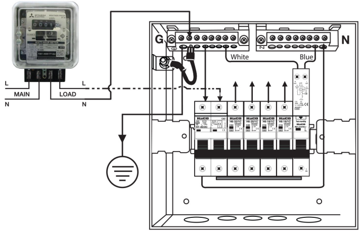
Main RCBO (RO7)
